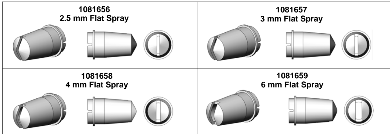
Figure 7-2 Flat Spray Nozzles
