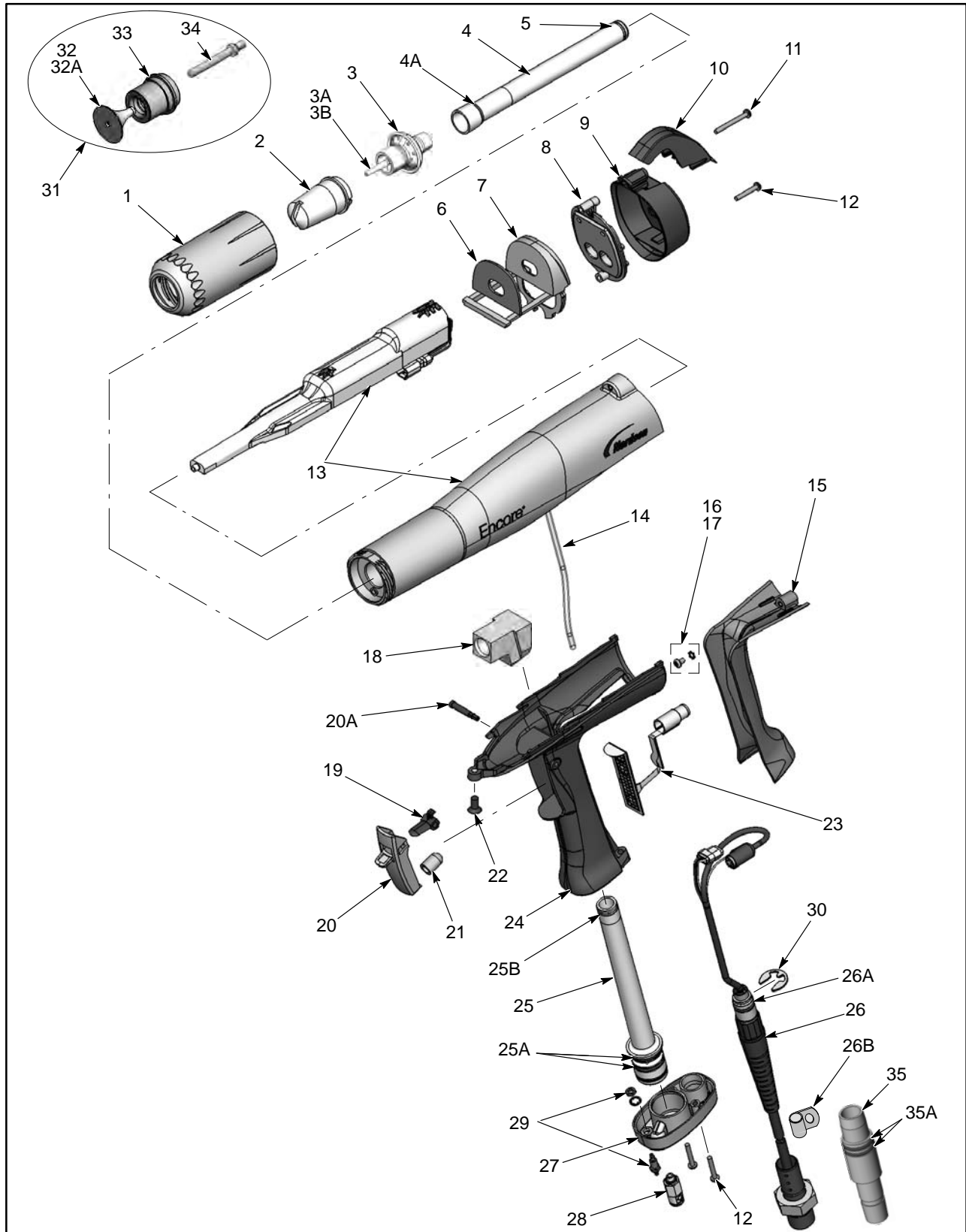
Figure 7-1 Exploded View of Encore LT Manual Spray Gun and Accessories
