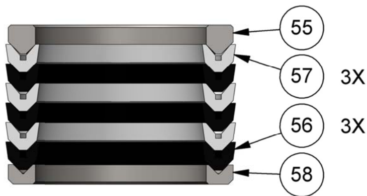
ITEM 39 Lower Packing Assembly
