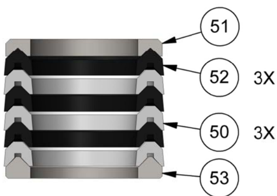
ITEM 28 Upper Packing Assembly
